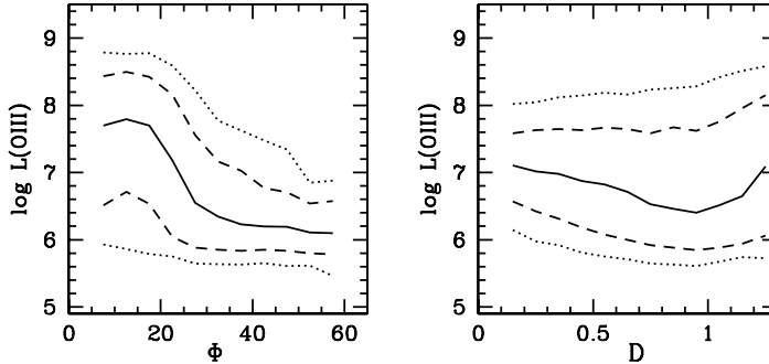
Figure 3: Left: The [OIII] line luminosity is plotted as a function of the angle parameter \Phi for all AGN lying above the Kewley et al. demarcation curve in Fig. 1. Right: The [OIII] line luminosity is plotted as a function of D , the distance from the locus of star-forming galaxies. In each plot the solid line shows the median relation as a function of D or \Phi , while the dashed and dotted lines indicate the 16-84 and 2.5-97.5 percentiles in \log L[\text{OIII}] respectively.
